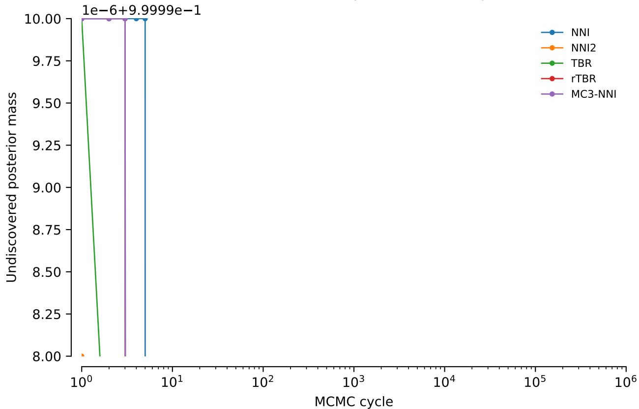
vert.nd3.tw5: Undiscovered posterior mass: power = 0.2
