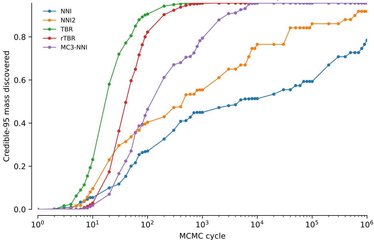
vert.nd3.tw5: Credible-95 mass discovered: power = 0.4
