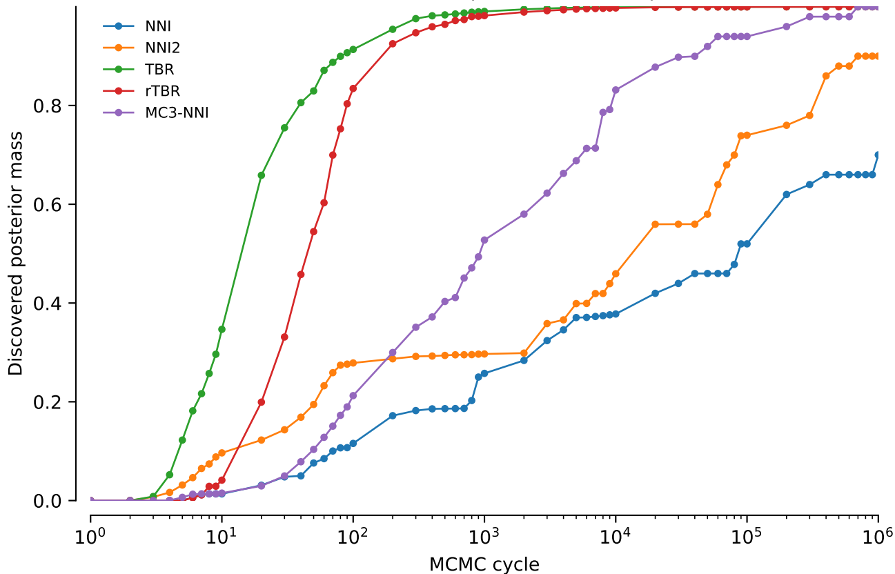
vert.nd3.tw5: Discovered posterior mass: power = 0.5
