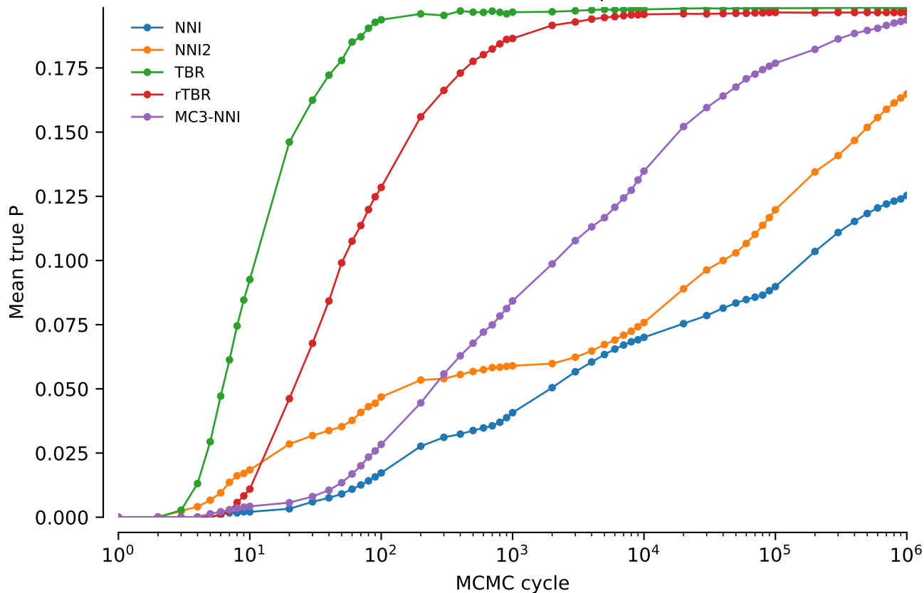
vert.nd3.tw5: Mean true P: power = 0.5
