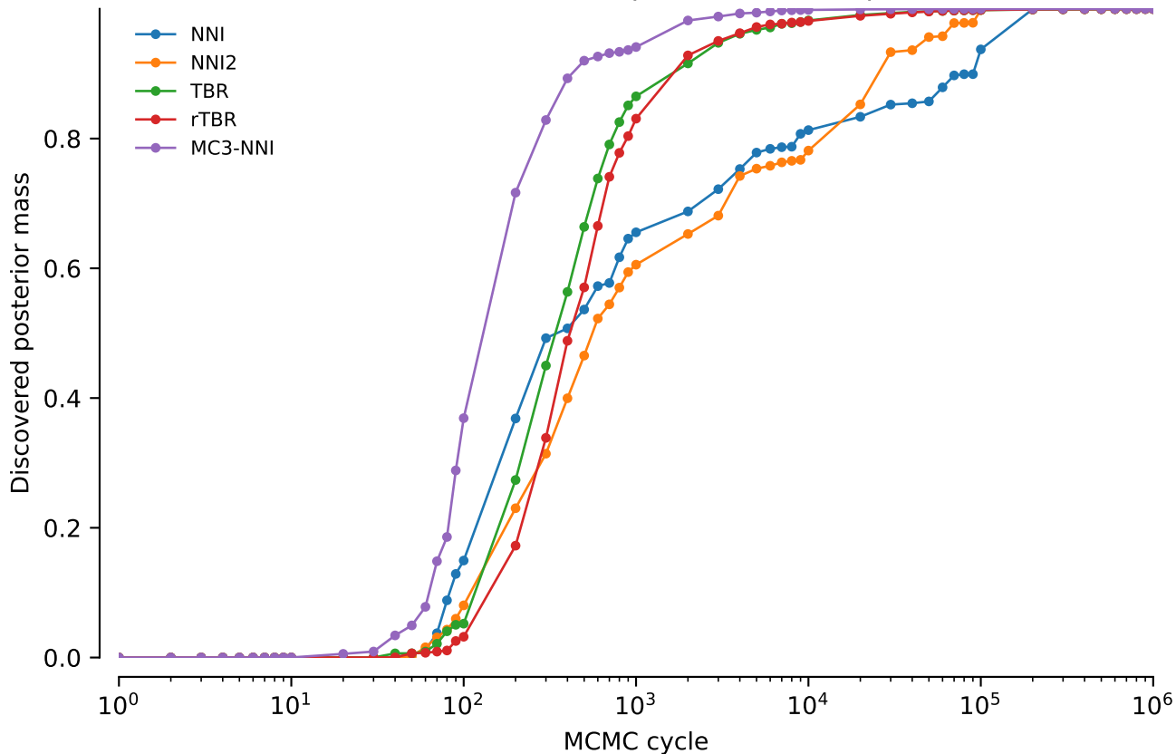
vert.nd3.tw5: Discovered posterior mass: power = 0
