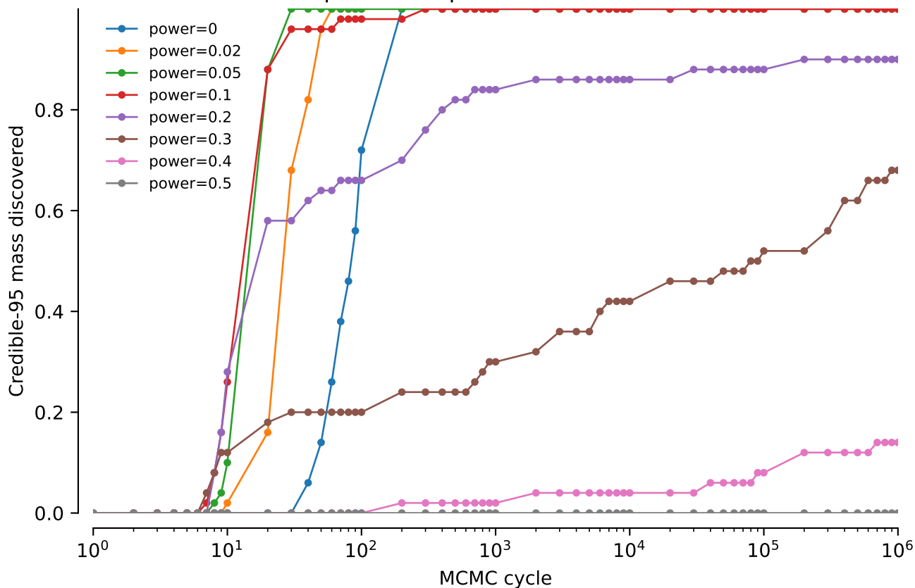
vert.nd4.tw0: NNI power comparison: Credible-95 mass discovered
