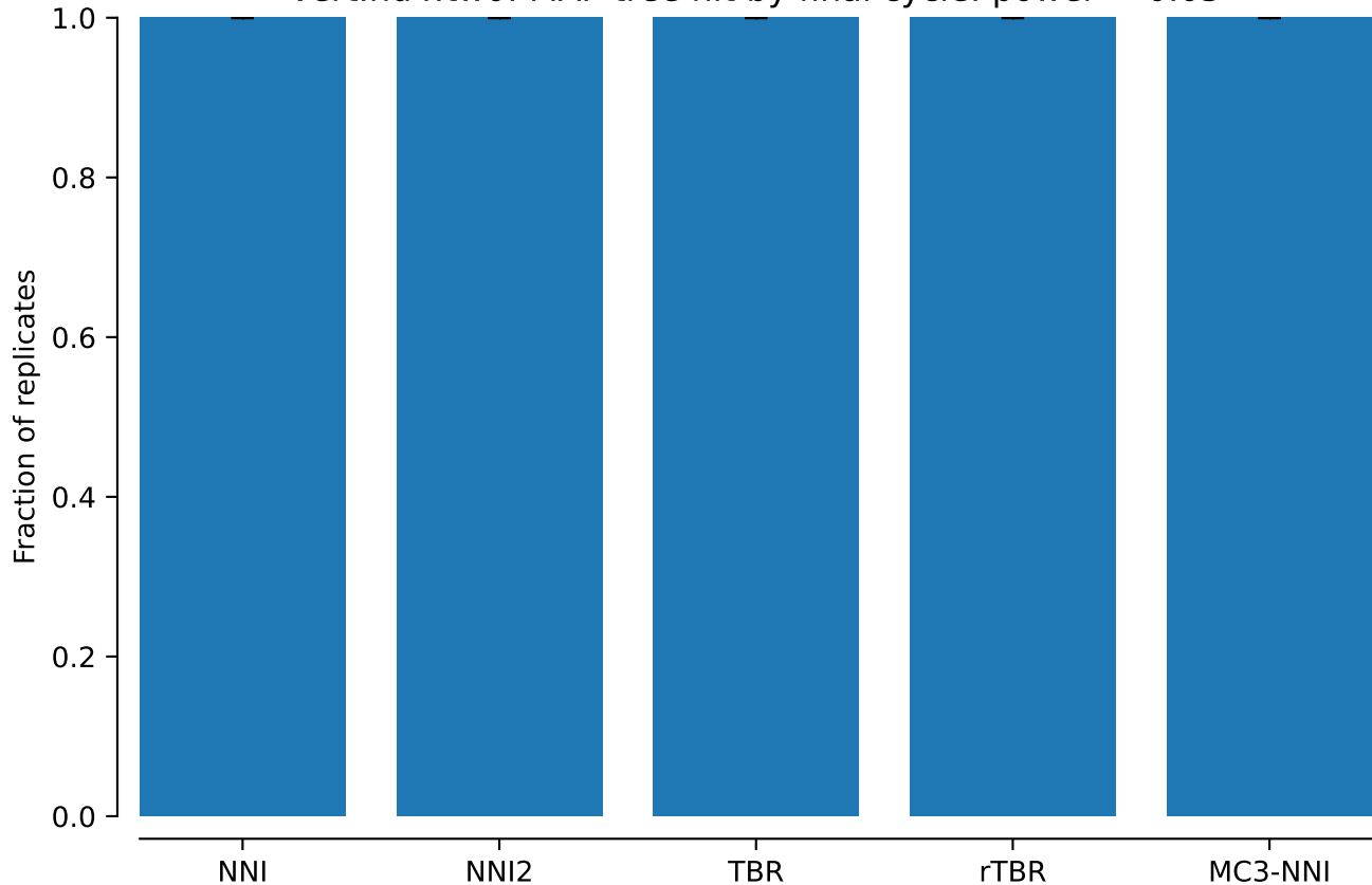
vert.nd4.tw0: MAP tree hit by final cycle: power = 0.05
