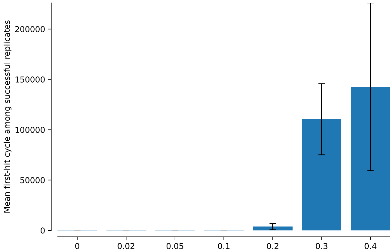
vert.nd4.tw0: NNI: mean MAP first-hit cycle
