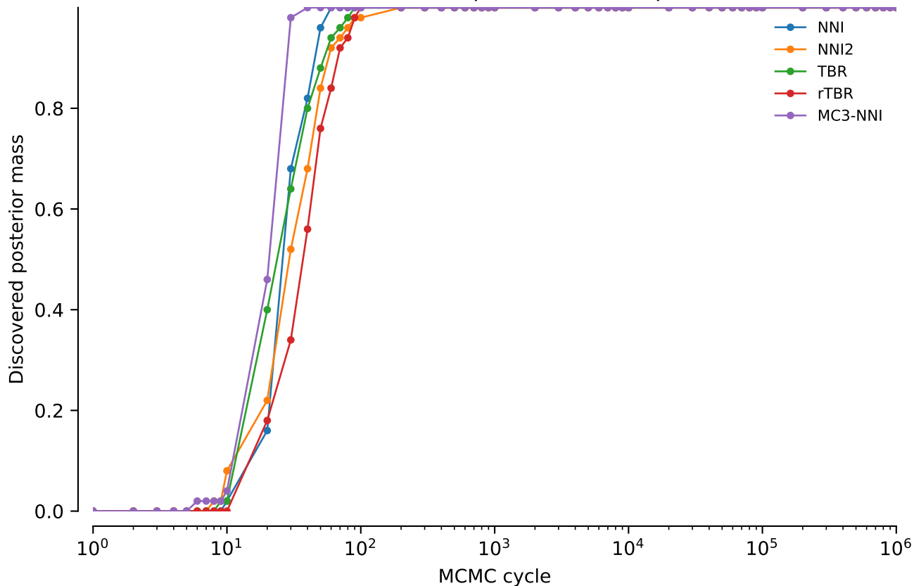
vert.nd4.tw0: Discovered posterior mass: power = 0.02
