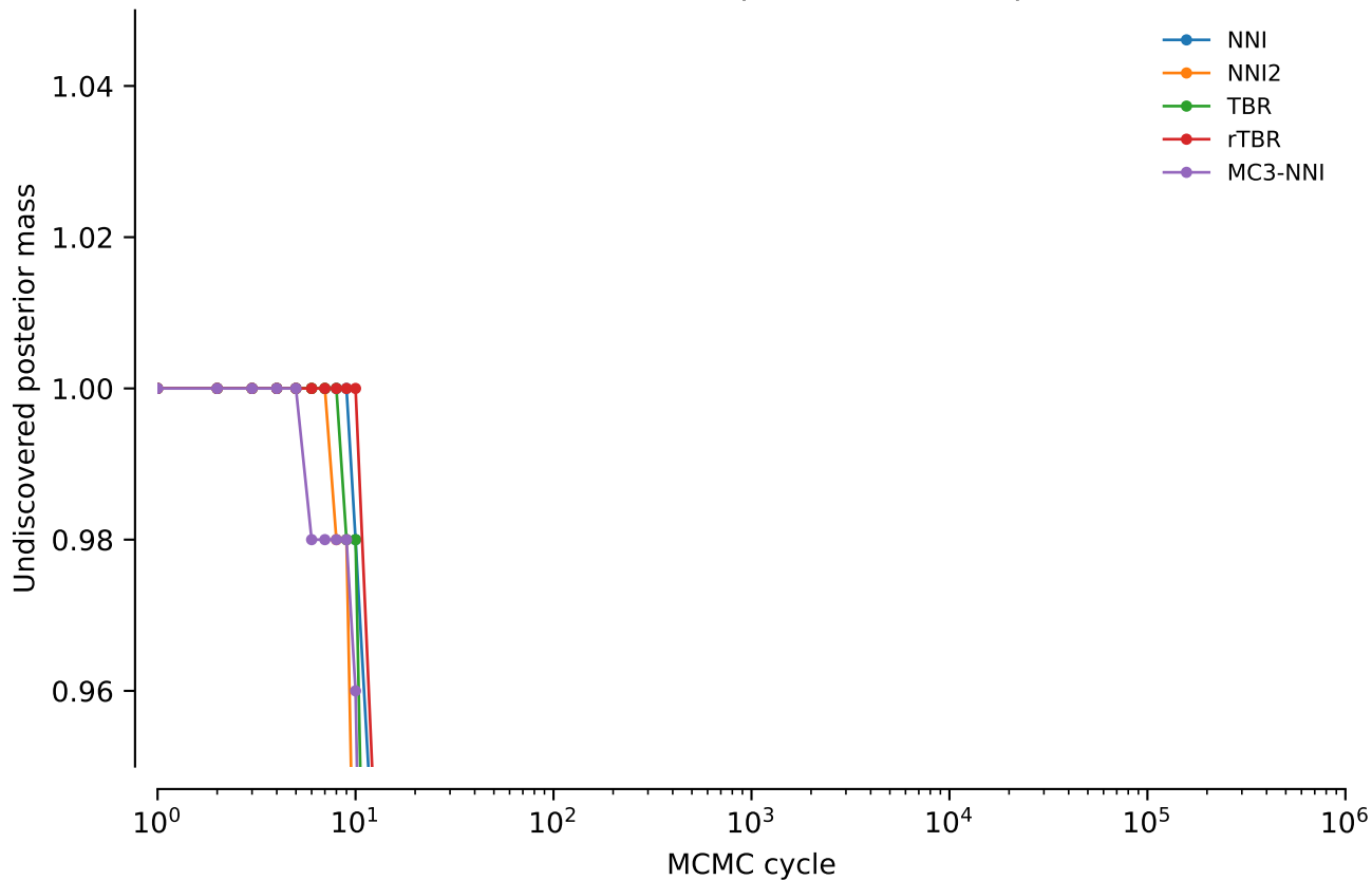
vert.nd4.tw0: Undiscovered posterior mass: power = 0.02
