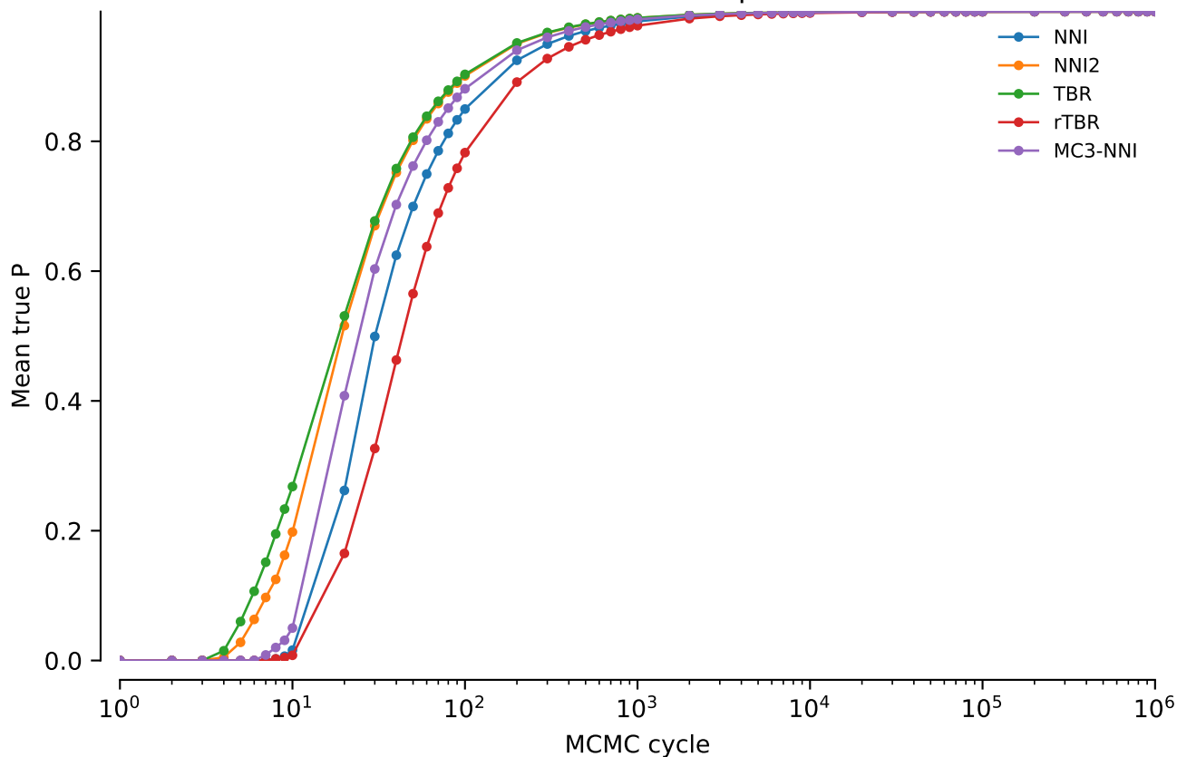
vert.nd4.tw0: Mean true P: power = 0.05
