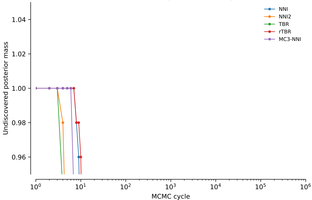
vert.nd4.tw0: Undiscovered posterior mass: power = 0.05
