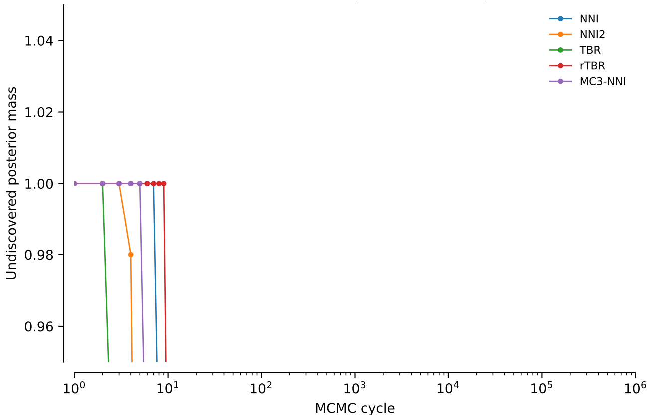
vert.nd4.tw0: Undiscovered posterior mass: power = 0.2
