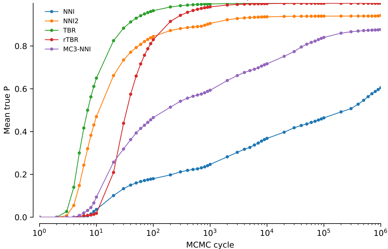
vert.nd4.tw0: Mean true P: power = 0.3
