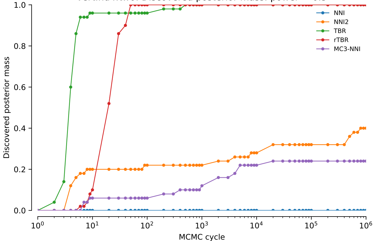
vert.nd4.tw0: Discovered posterior mass: power = 0.5
