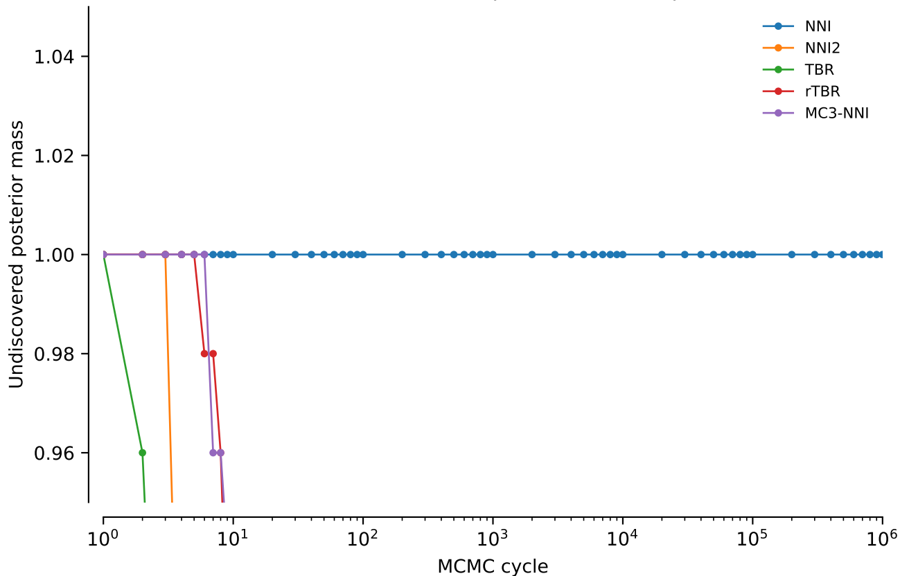
vert.nd4.tw0: Undiscovered posterior mass: power = 0.5
