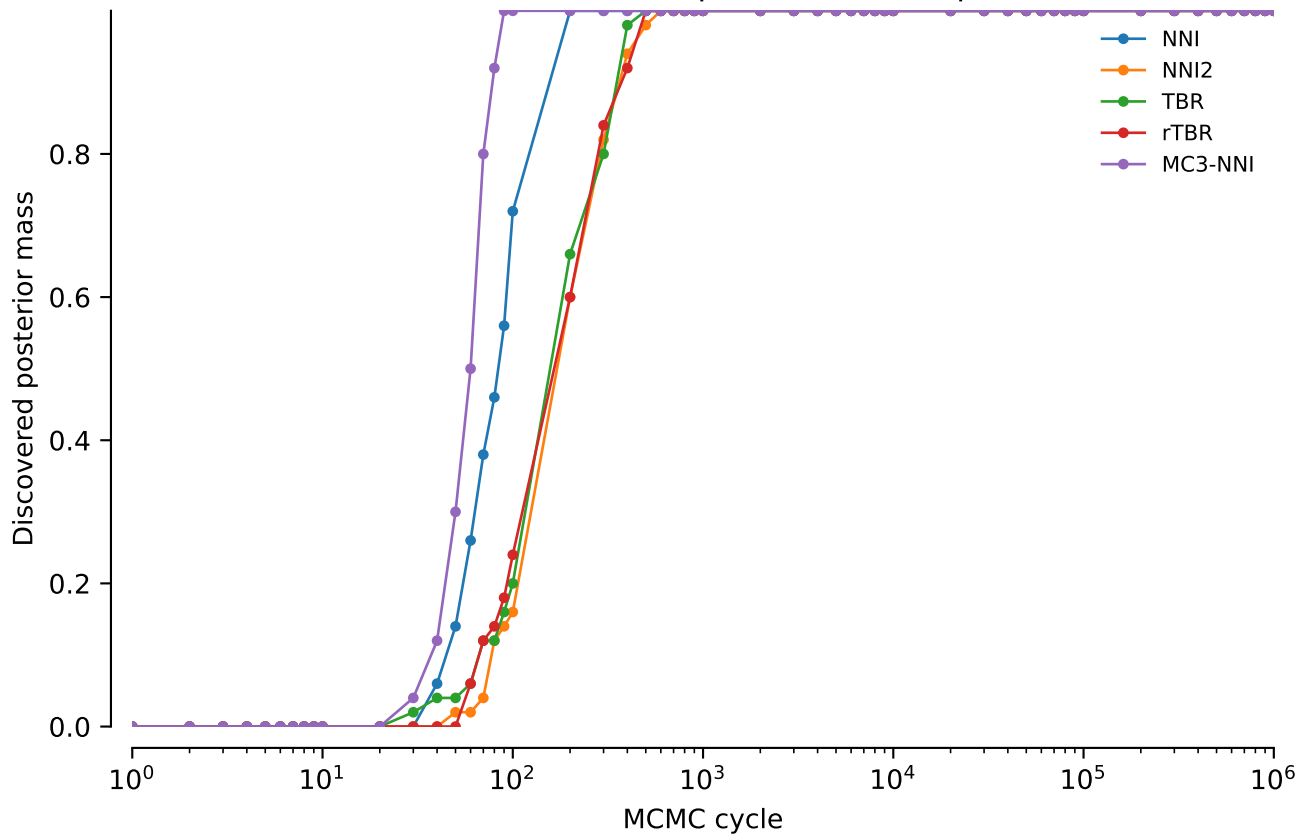
vert.nd4.tw0: Discovered posterior mass: power = 0
