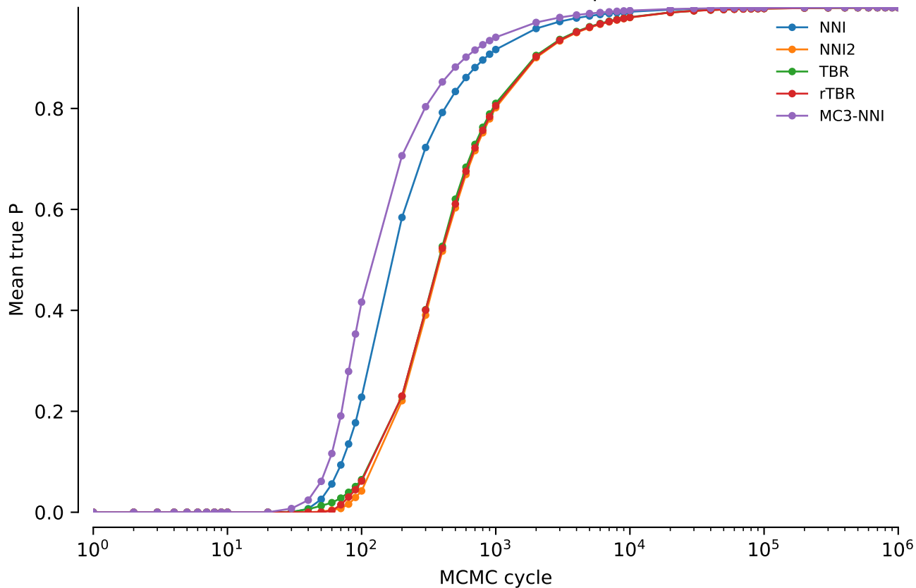
vert.nd4.tw0: Mean true P: power = 0
