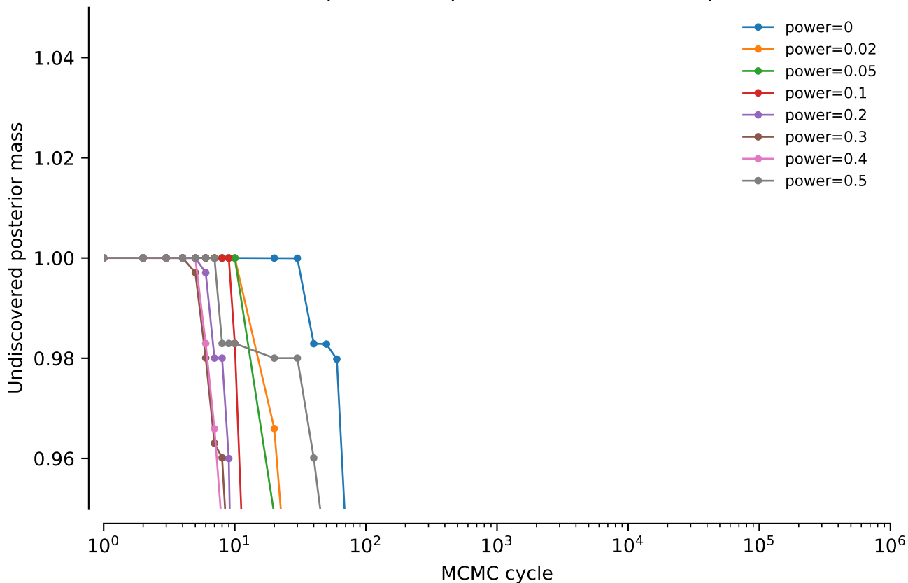
vert.nd4.tw5: NNI power comparison: Undiscovered posterior mass
