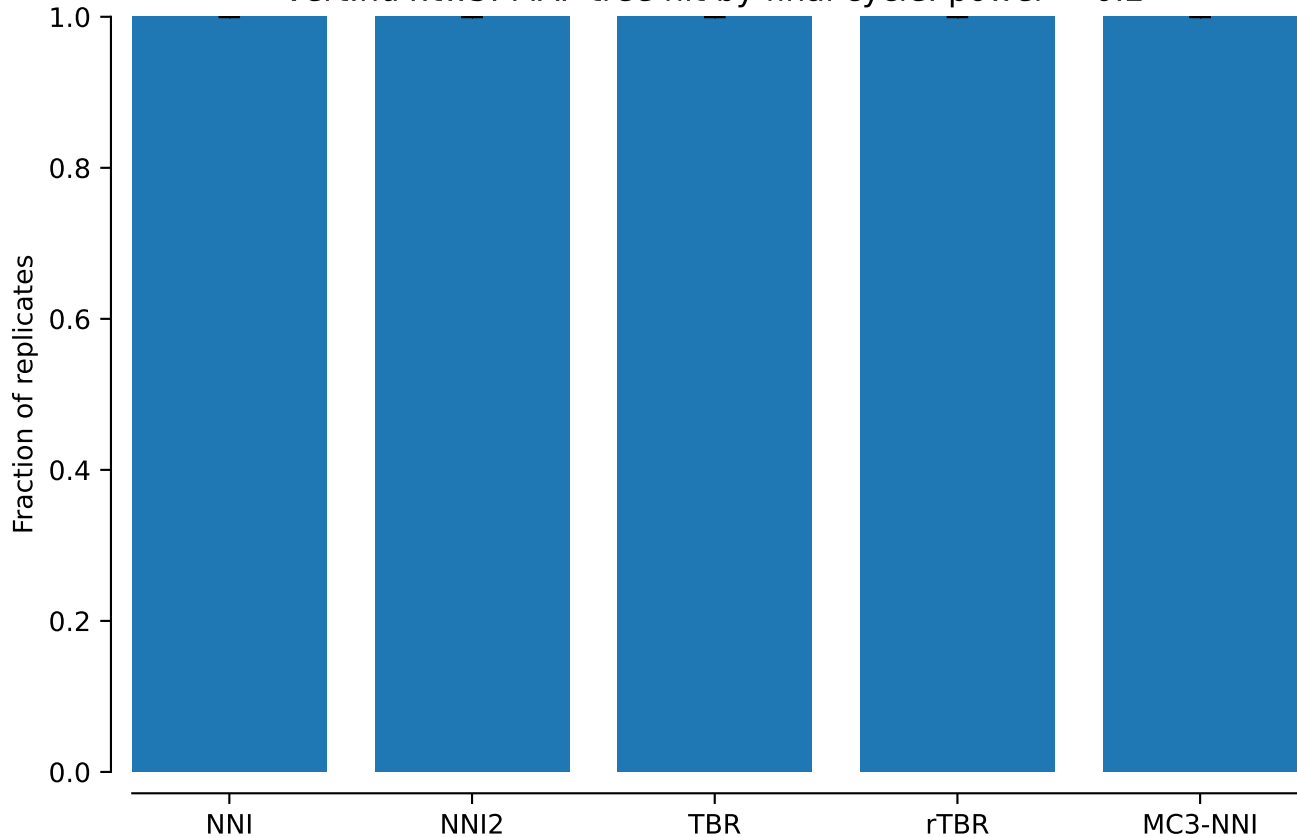
vert.nd4.tw5: MAP tree hit by final cycle: power = 0.2
