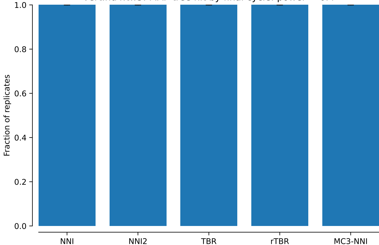
vert.nd4.tw5: MAP tree hit by final cycle: power = 0.4
