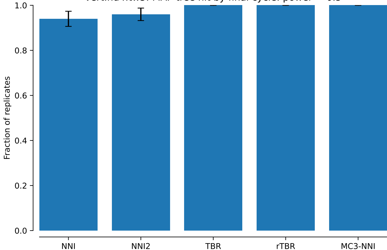
vert.nd4.tw5: MAP tree hit by final cycle: power = 0.5
