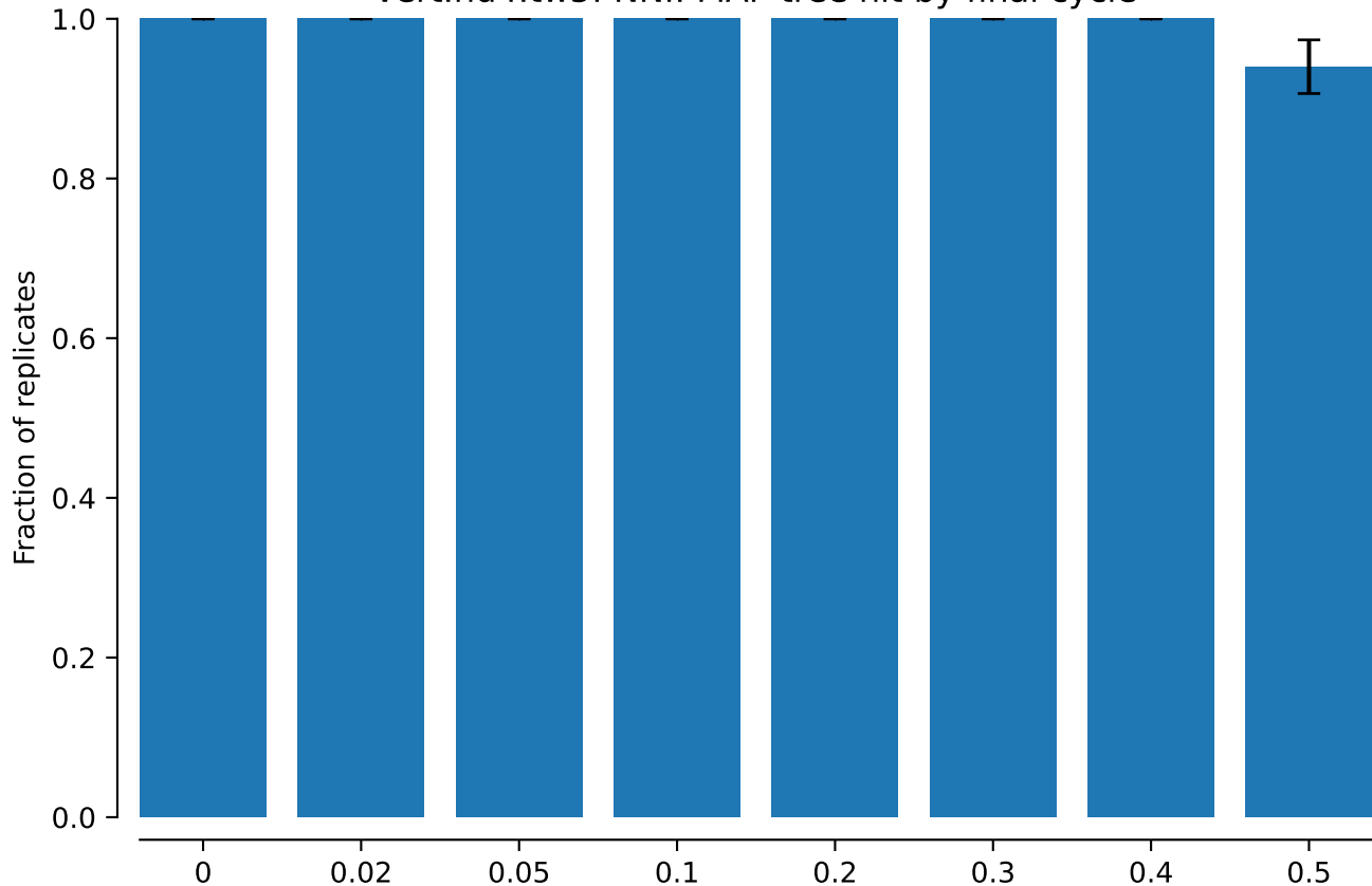
vert.nd4.tw5: NNI: MAP tree hit by final cycle
