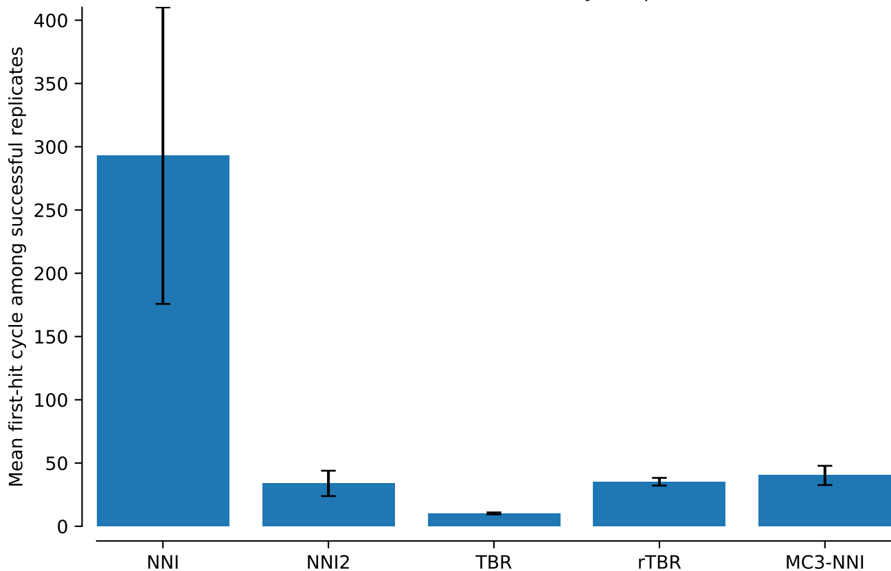
vert.nd4.tw5: Mean MAP first-hit cycle: power = 0.3
