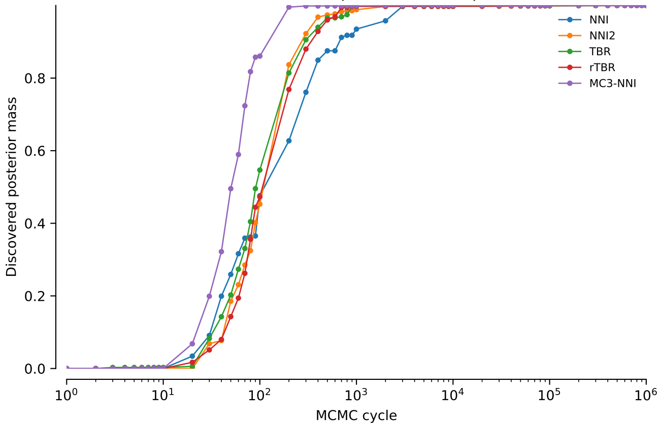
vert.nd4.tw5: Discovered posterior mass: power = 0.02
