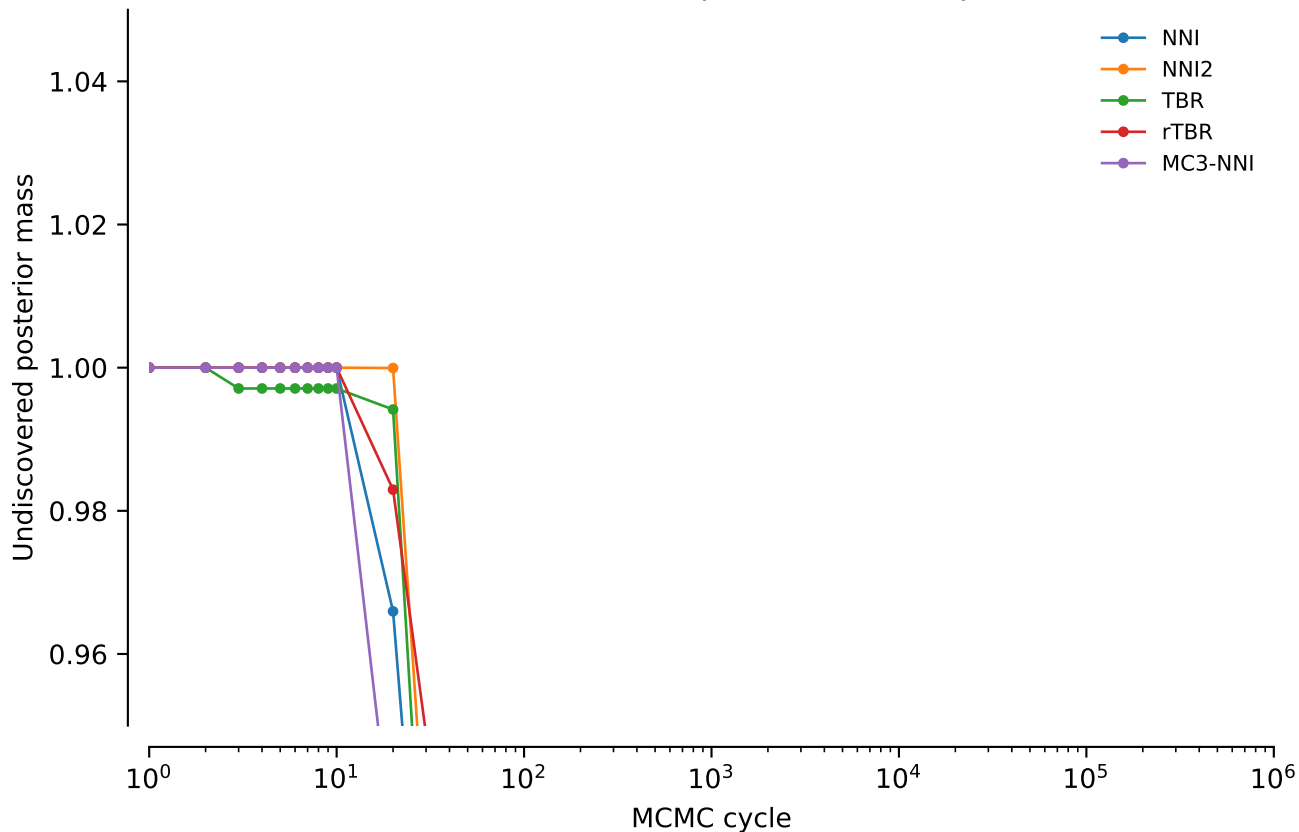
vert.nd4.tw5: Undiscovered posterior mass: power = 0.02
