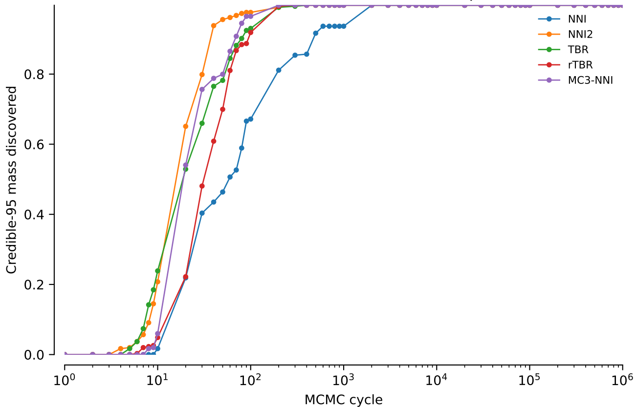
vert.nd4.tw5: Credible-95 mass discovered: power = 0.1
