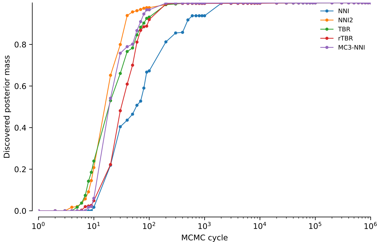
vert.nd4.tw5: Discovered posterior mass: power = 0.1
