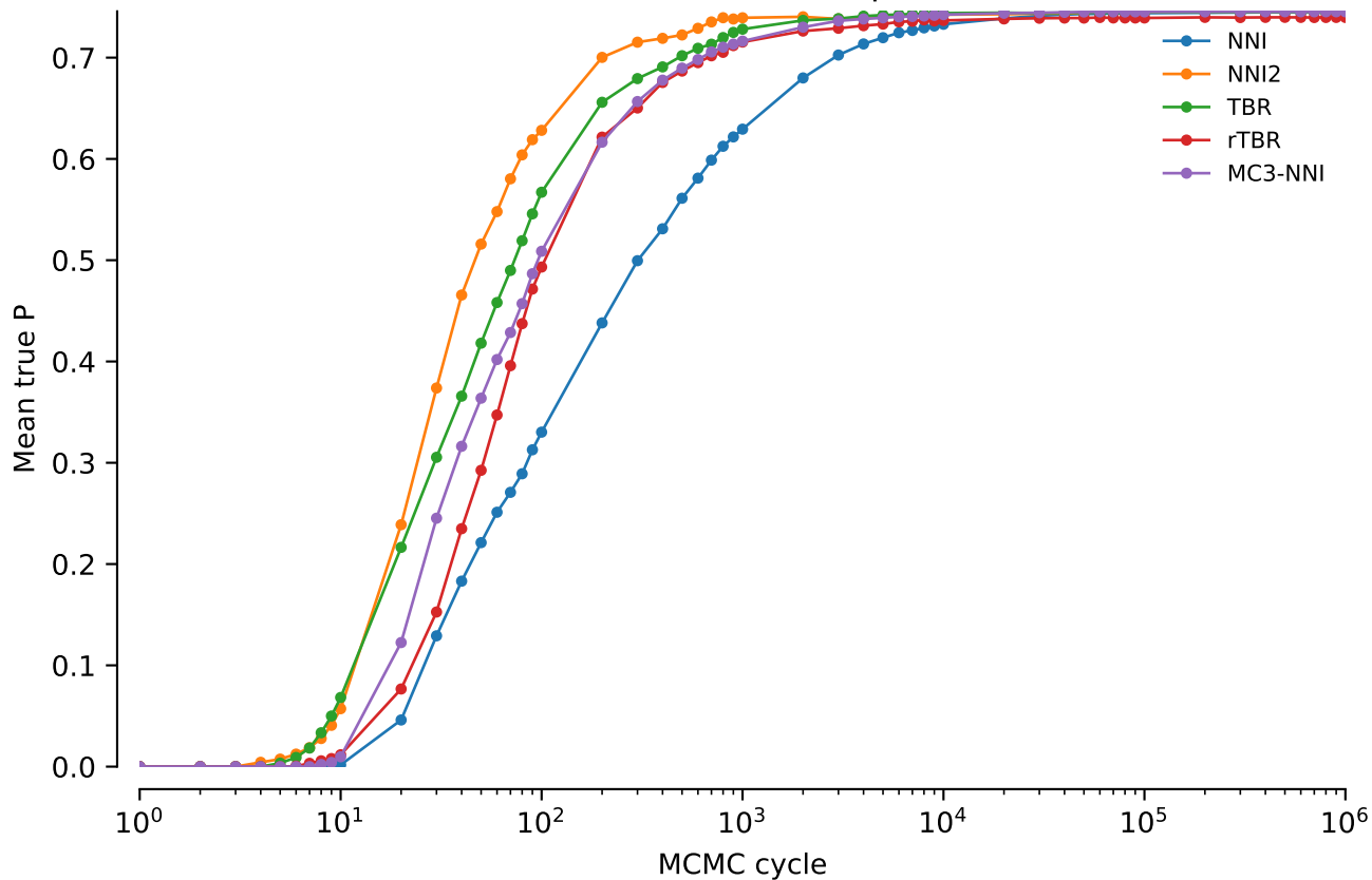
vert.nd4.tw5: Mean true P: power = 0.1
