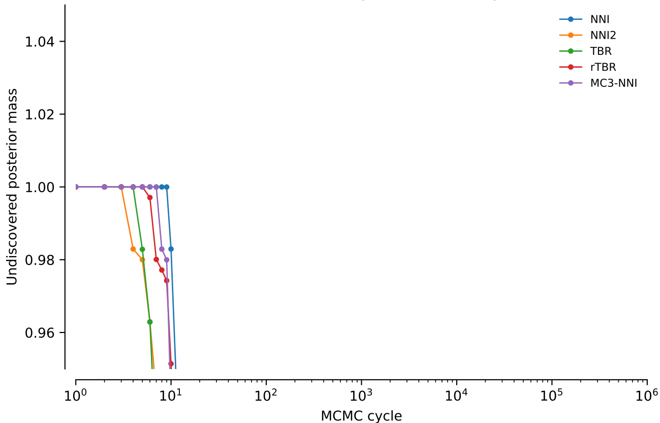
vert.nd4.tw5: Undiscovered posterior mass: power = 0.1
