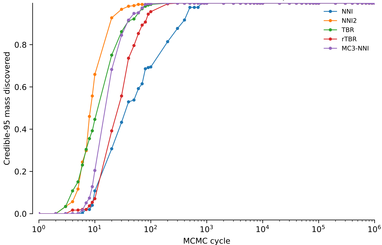
vert.nd4.tw5: Credible-95 mass discovered: power = 0.2
