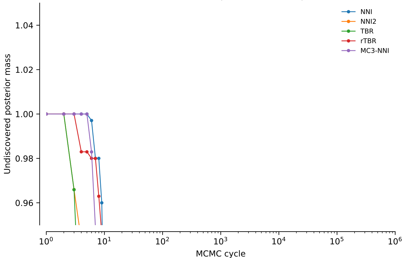
vert.nd4.tw5: Undiscovered posterior mass: power = 0.2
