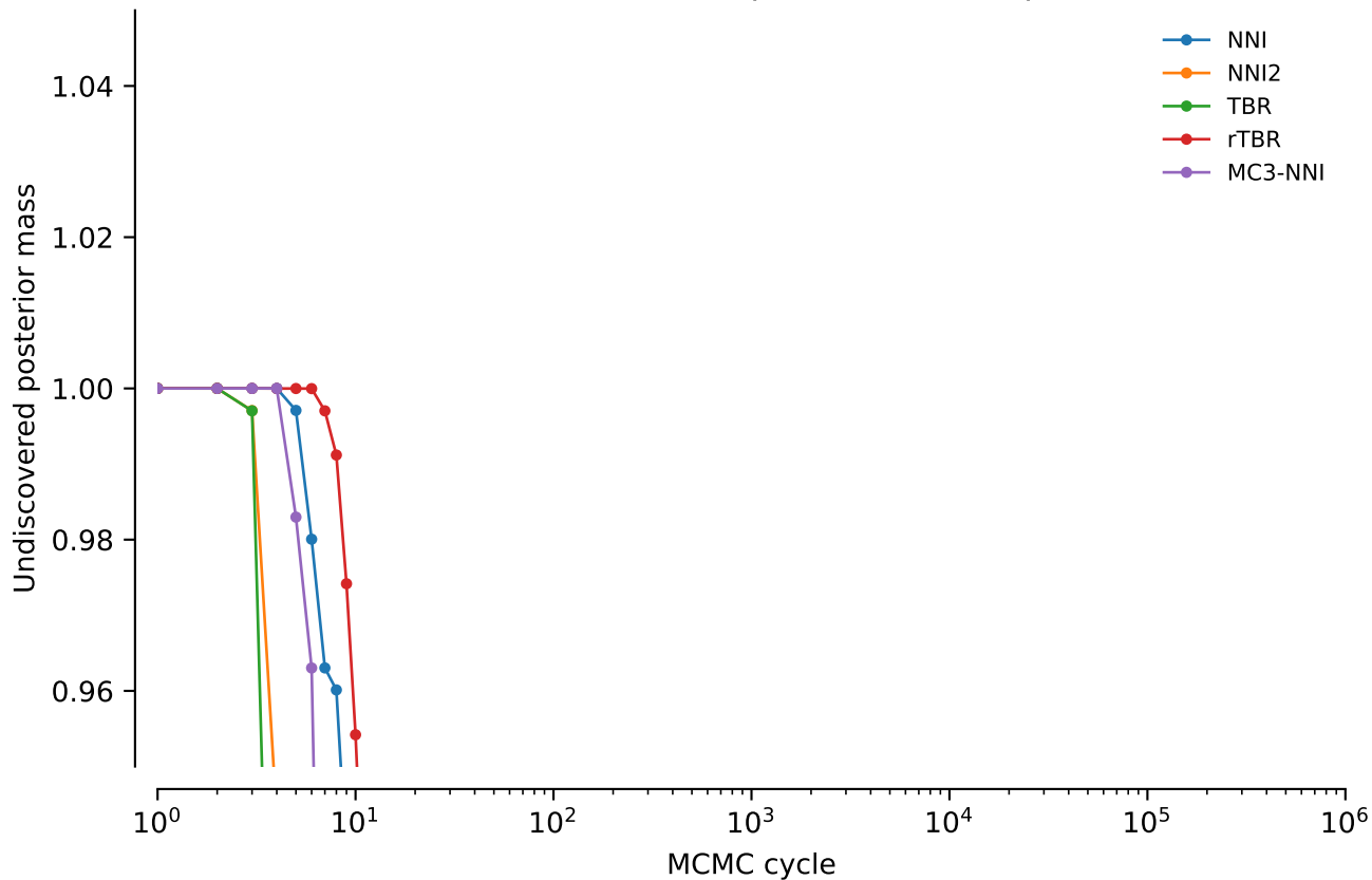
vert.nd4.tw5: Undiscovered posterior mass: power = 0.3
