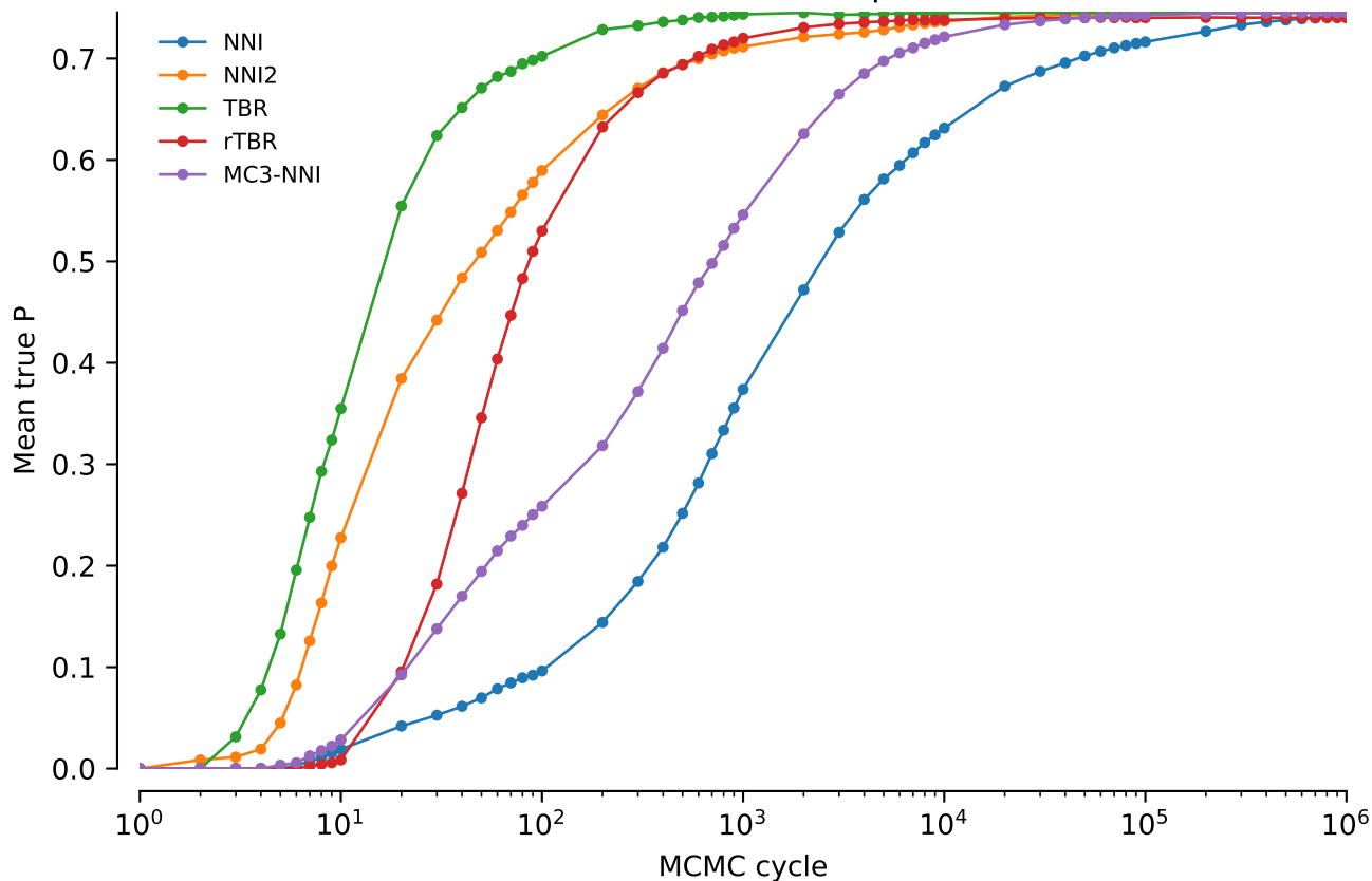
vert.nd4.tw5: Mean true P: power = 0.4
