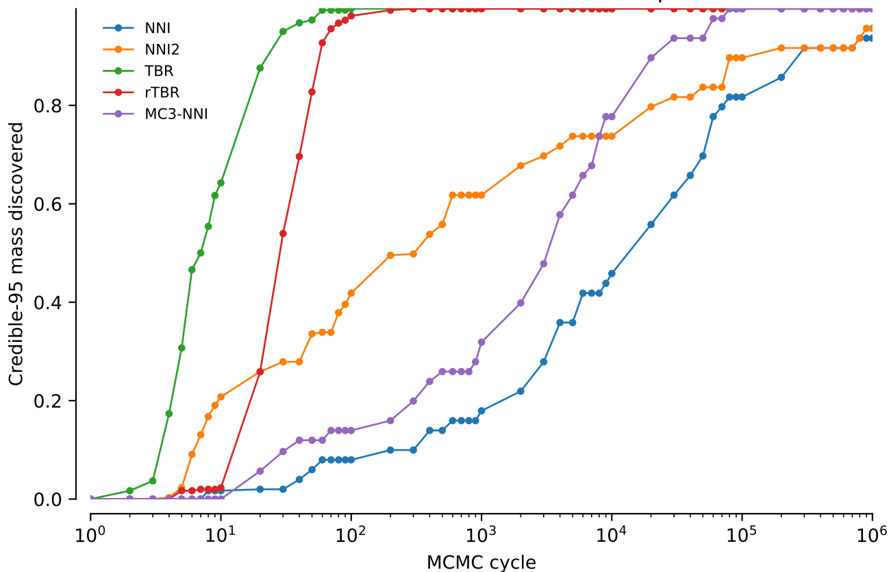
vert.nd4.tw5: Credible-95 mass discovered: power = 0.5
