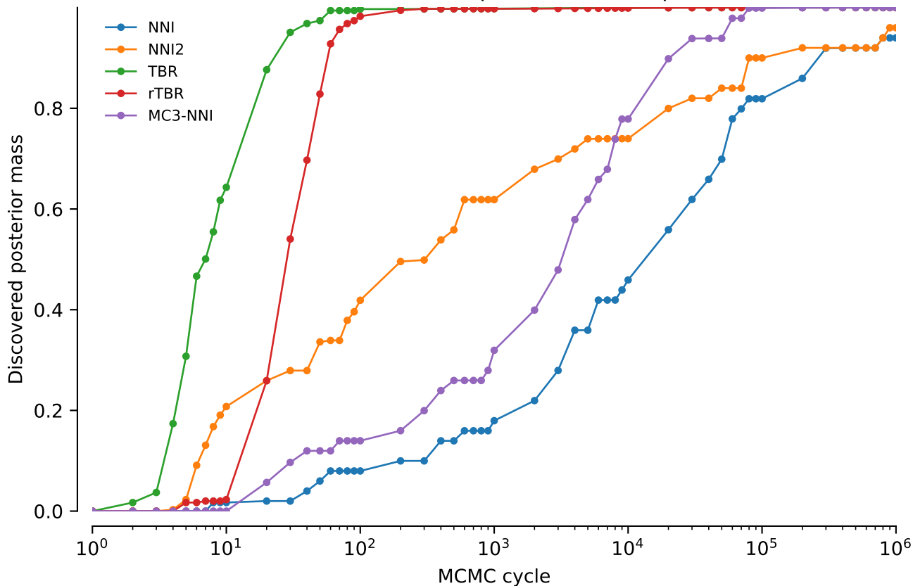
vert.nd4.tw5: Discovered posterior mass: power = 0.5
