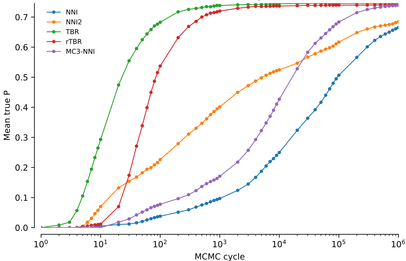
vert.nd4.tw5: Mean true P: power = 0.5
