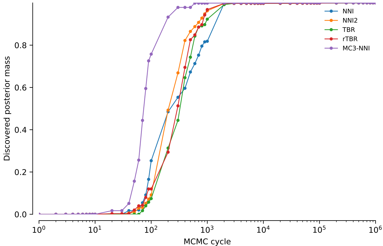
vert.nd4.tw5: Discovered posterior mass: power = 0
