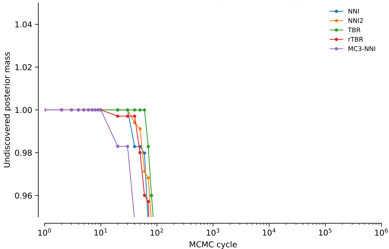
vert.nd4.tw5: Undiscovered posterior mass: power = 0
