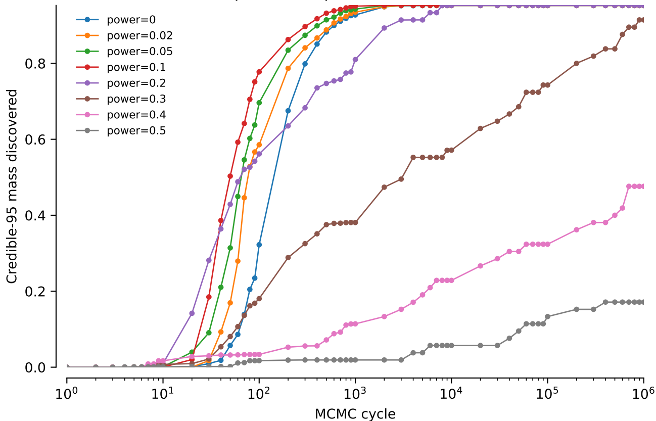
vert.nd4l.tw0: NNI power comparison: Credible-95 mass discovered
