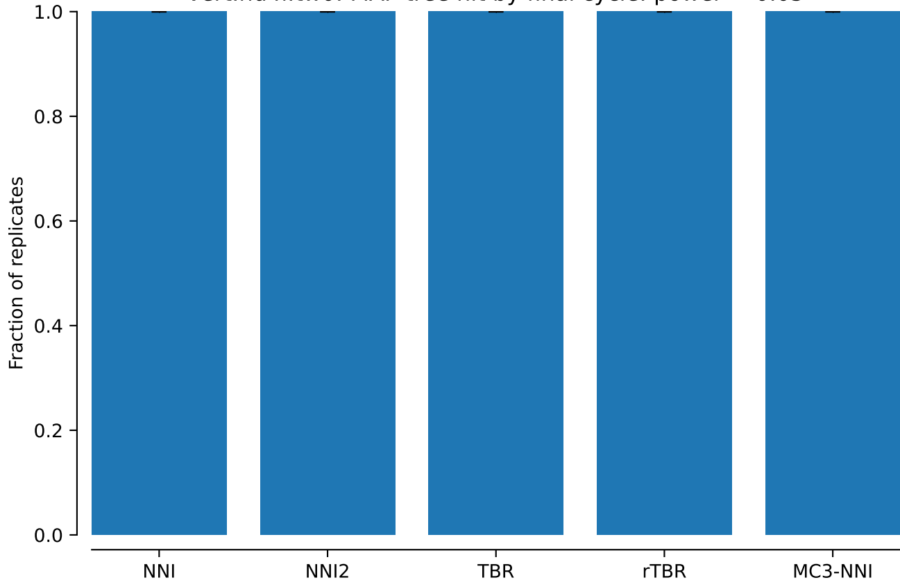
vert.nd4l.tw0: MAP tree hit by final cycle: power = 0.05
