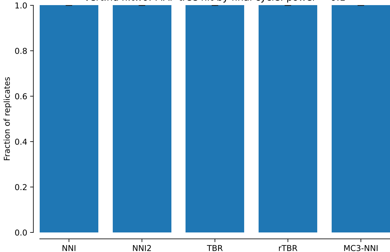
vert.nd4l.tw0: MAP tree hit by final cycle: power = 0.1
