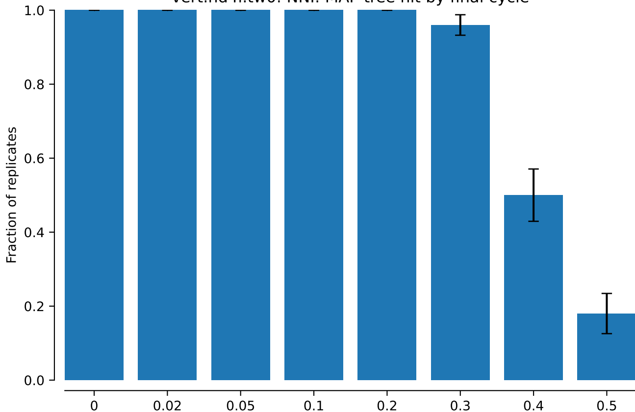
vert.nd4l.tw0: NNI: MAP tree hit by final cycle
