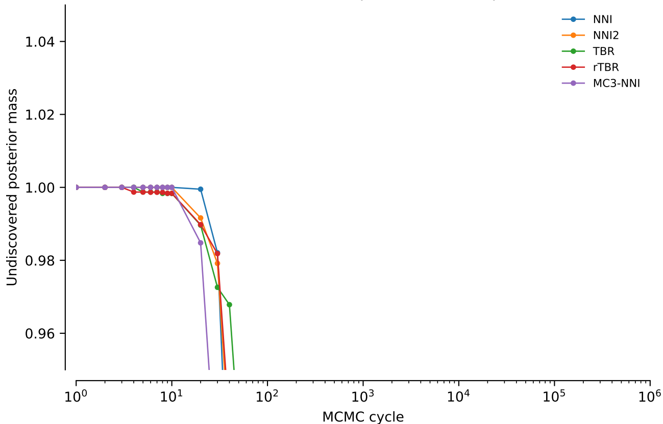
vert.nd4l.tw0: Undiscovered posterior mass: power = 0.02
