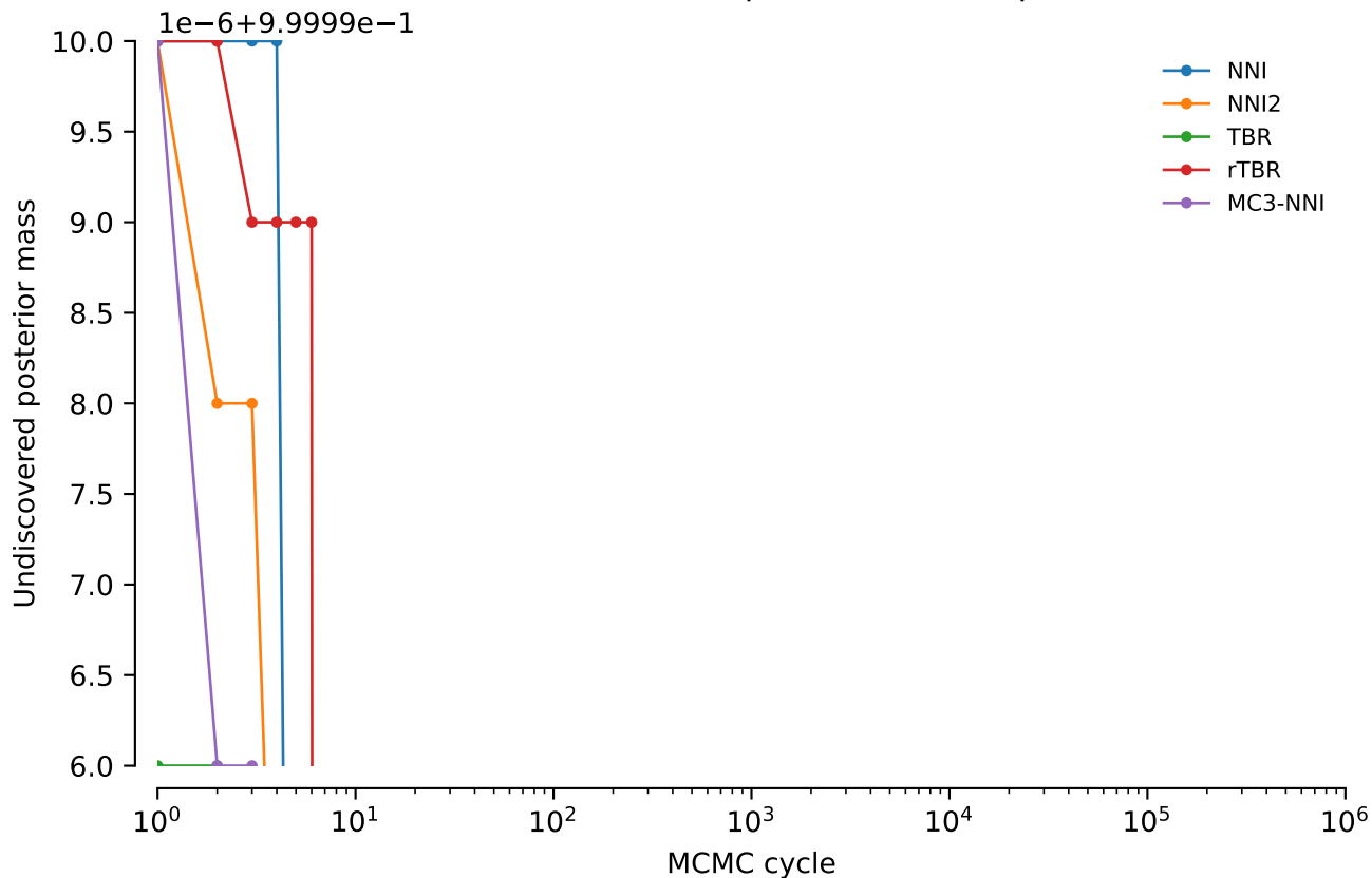
vert.nd4l.tw0: Undiscovered posterior mass: power = 0.05
