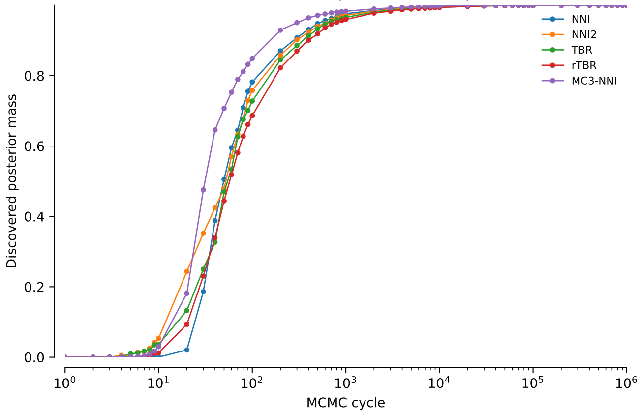
vert.nd4l.tw0: Discovered posterior mass: power = 0.1
