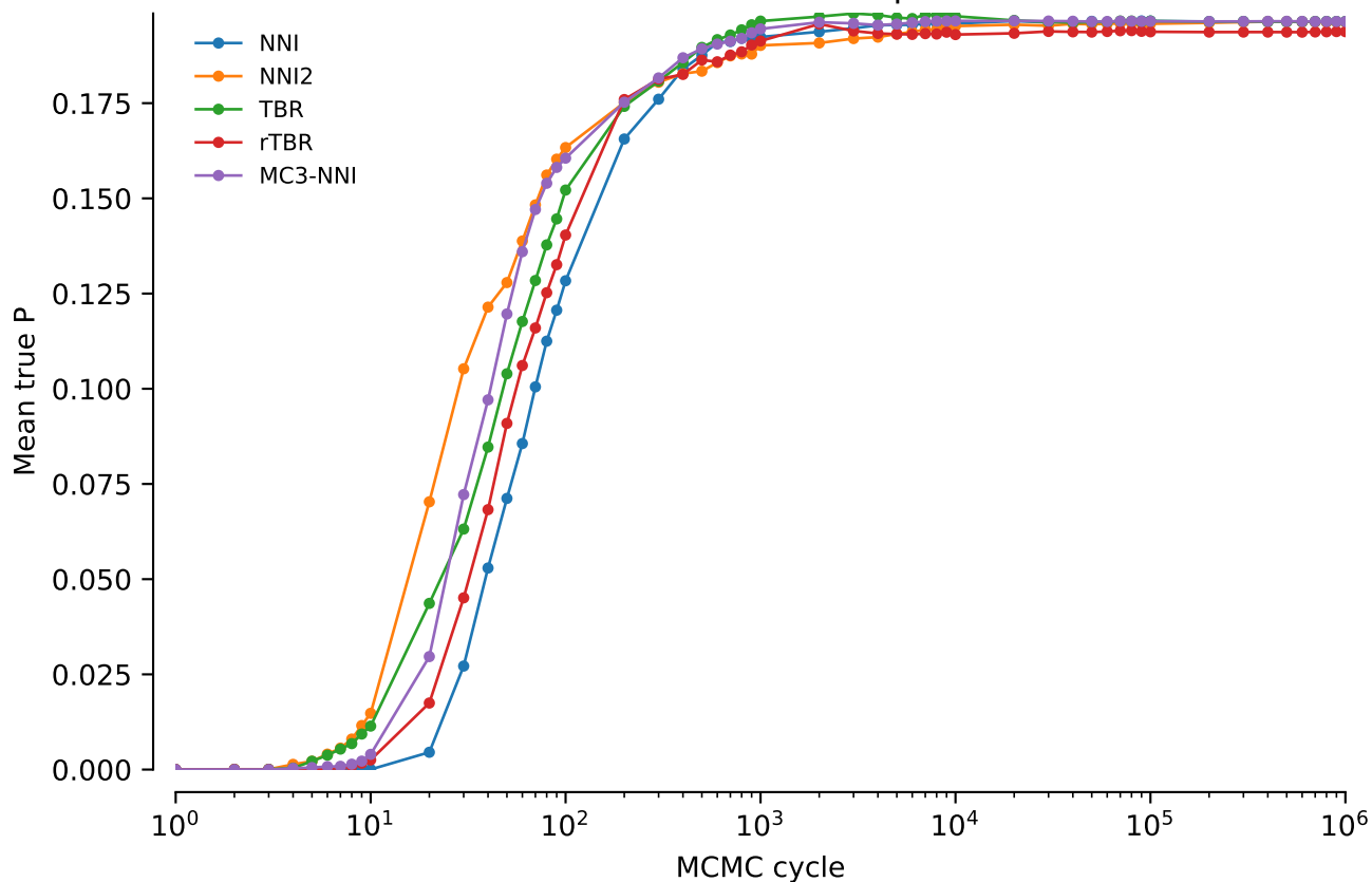
vert.nd4l.tw0: Mean true P: power = 0.1
