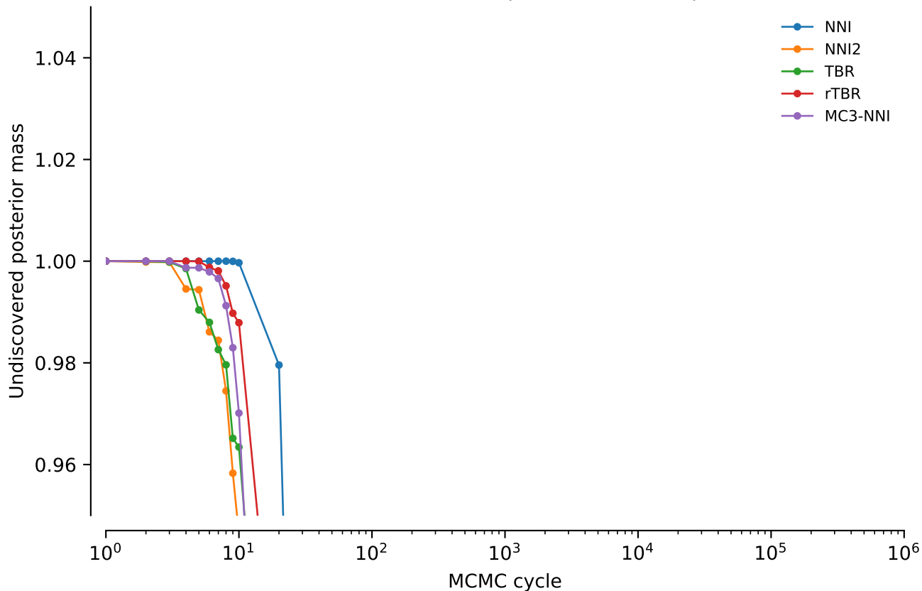
vert.nd4l.tw0: Undiscovered posterior mass: power = 0.1
