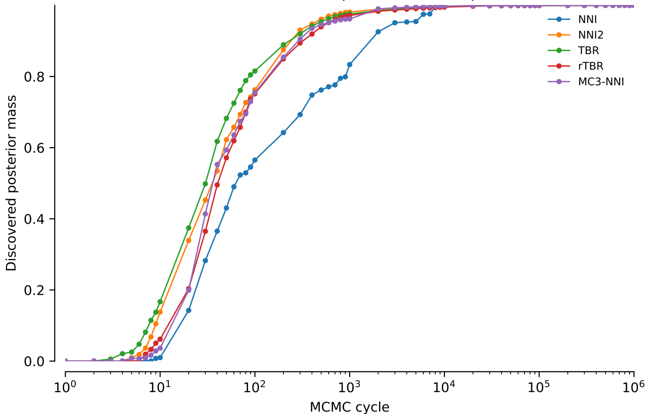
vert.nd4l.tw0: Discovered posterior mass: power = 0.2
