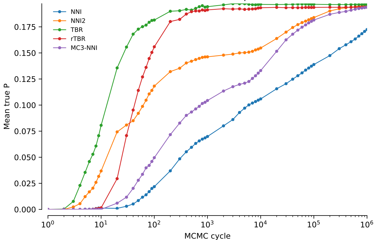
vert.nd4l.tw0: Mean true P: power = 0.3
